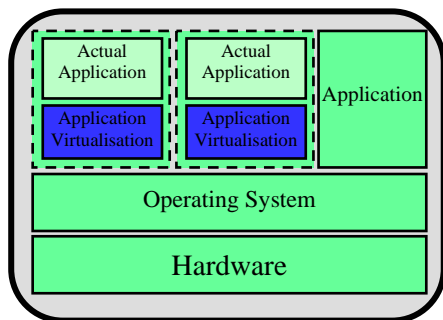
Figure 3 – Application Virtualisation
